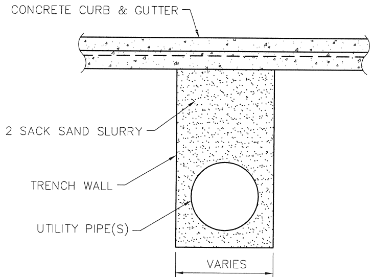
UTILITY TRENCH CUT-OFF WALL END VIEW
